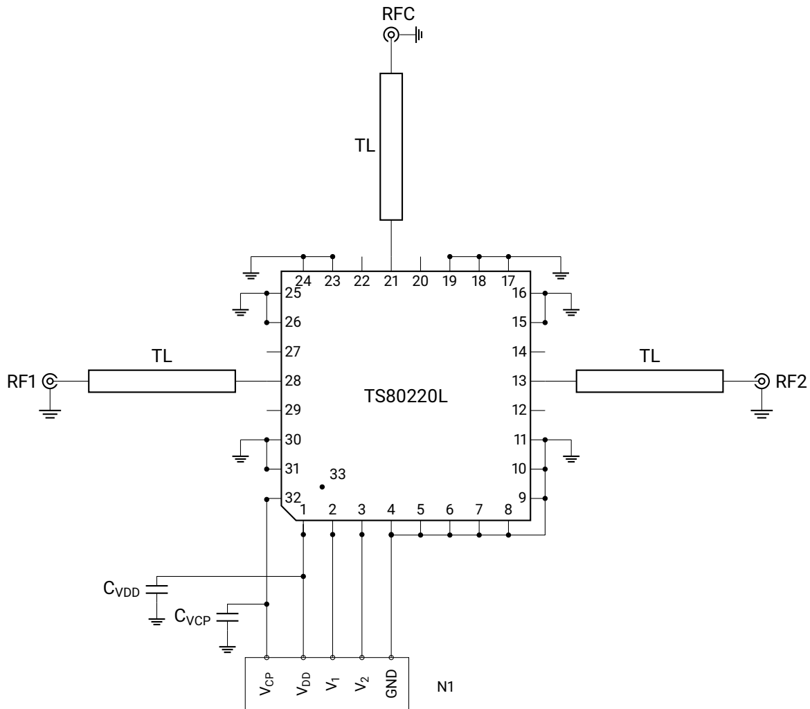
Schematics of TS80220L EVB
