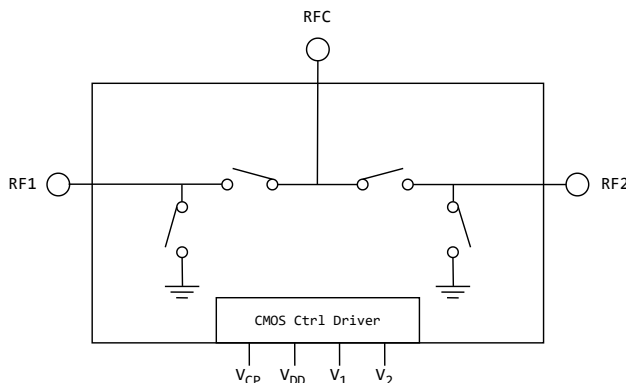
Figure 2: TS80220L functional diagram
